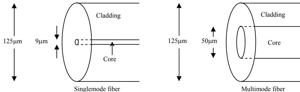
Figure 1: Optical Fibers
