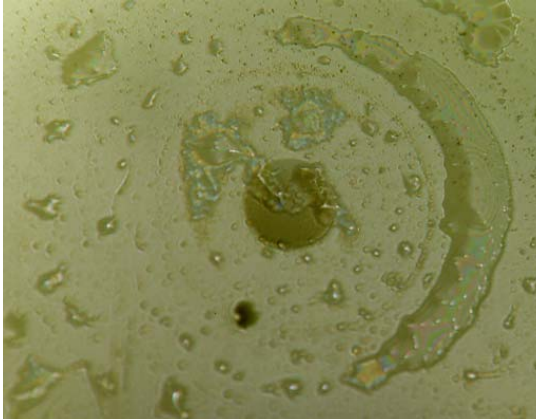
Ceramic ferrule showing RI liquid contamination
