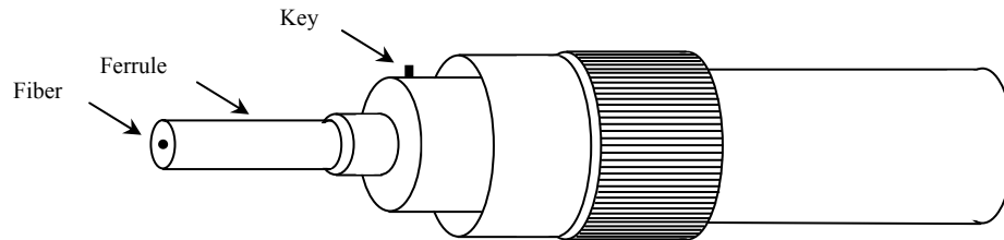
Figure 2: Optical Connector
